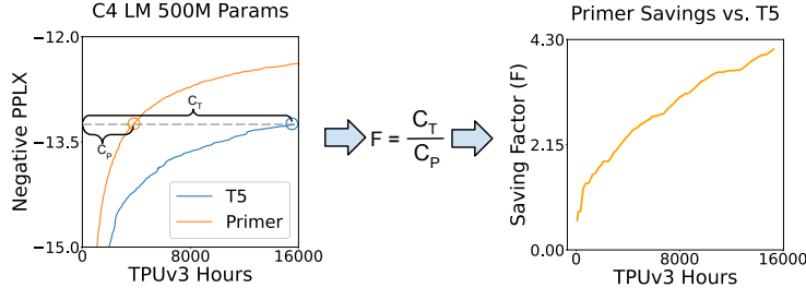
Figure 10: Compute savings of Primer vs. the original T5 architecture on C4 LM over time. The more compute invested in training, the higher the savings due to the asymptotic nature of both perplexity curves. Primer achieves the same performance as the original T5 architecture with 4.2X less compute.
